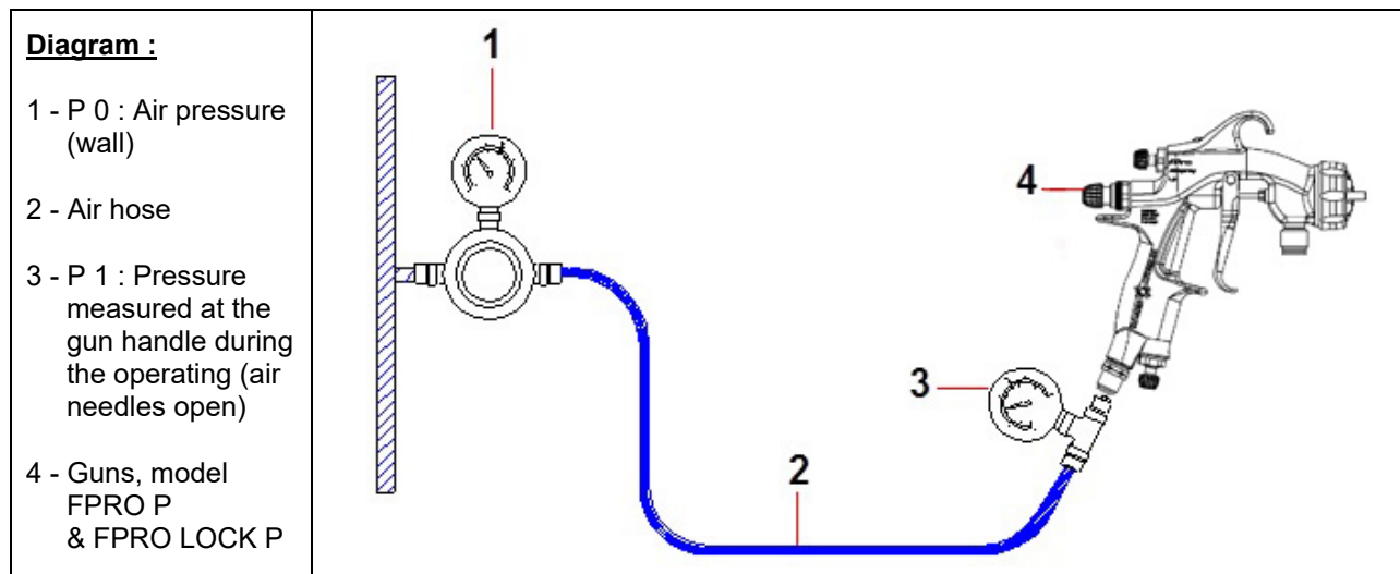
Gun, model FPRO P LP + HVLP aircap + hose Ø 8 mm, 7.5 m / 24.6 ft length
