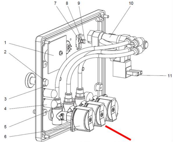
Motor-driven valves
